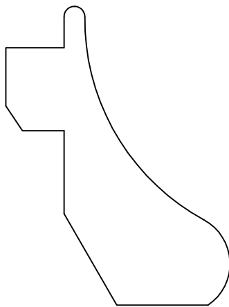
GM-4602 7/8" X 2 1/2"
