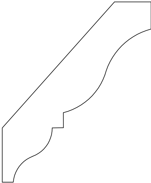
GM-4137 3/4" X 3 29/32"
