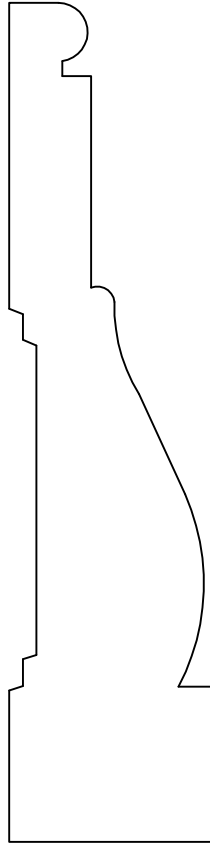
GM-3062 1 1/16" X 4 3/8"
