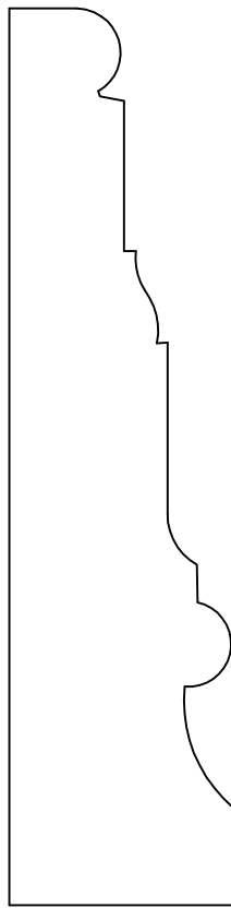
GM-3060 1 1/16" X 4 1/4"
