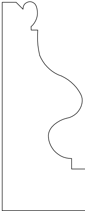
GM-3048 1 1/2" X 3 3/4"
