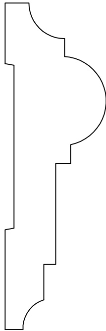
GM-2122 1 1/16" X 3 1/2"
