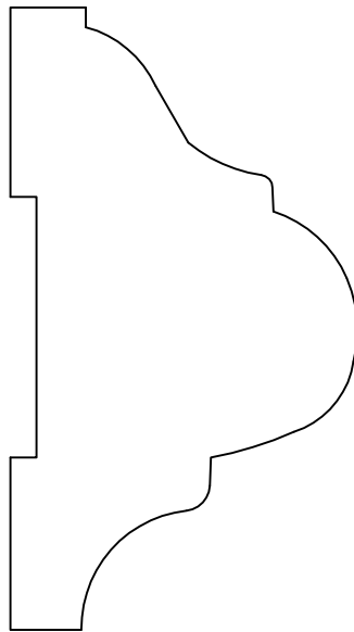
GM-2117 1 11/16" X 3"
