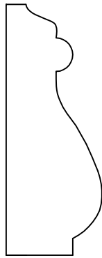
GM-1549-19 3/4" X 1 7/8"
